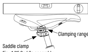
Fig. 4/15 Saddle assembly
