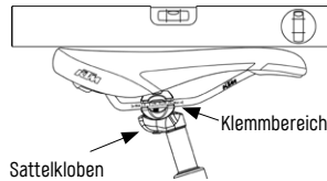
Abb. 4/15 Sattelmontage
